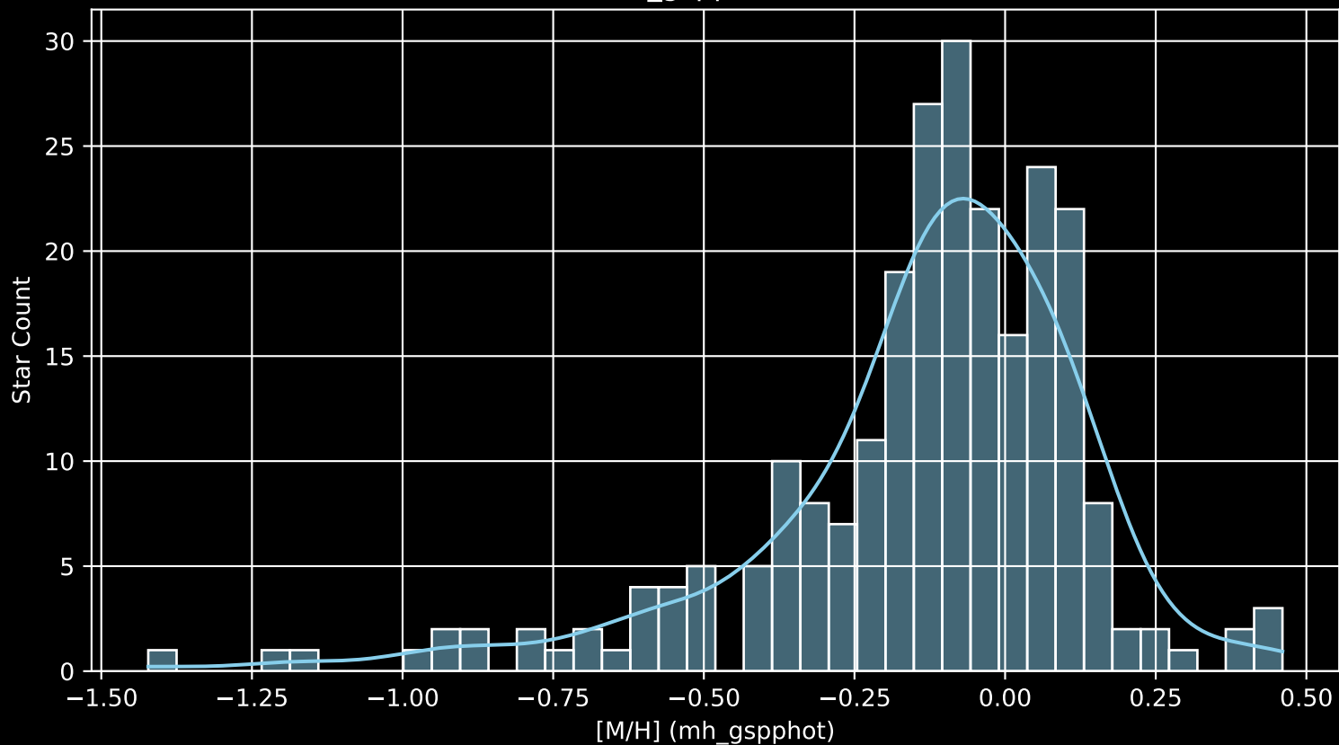
APOGEE DR17 Field: [005+12 [M/H] (mh_gspphot) (n= 246)
