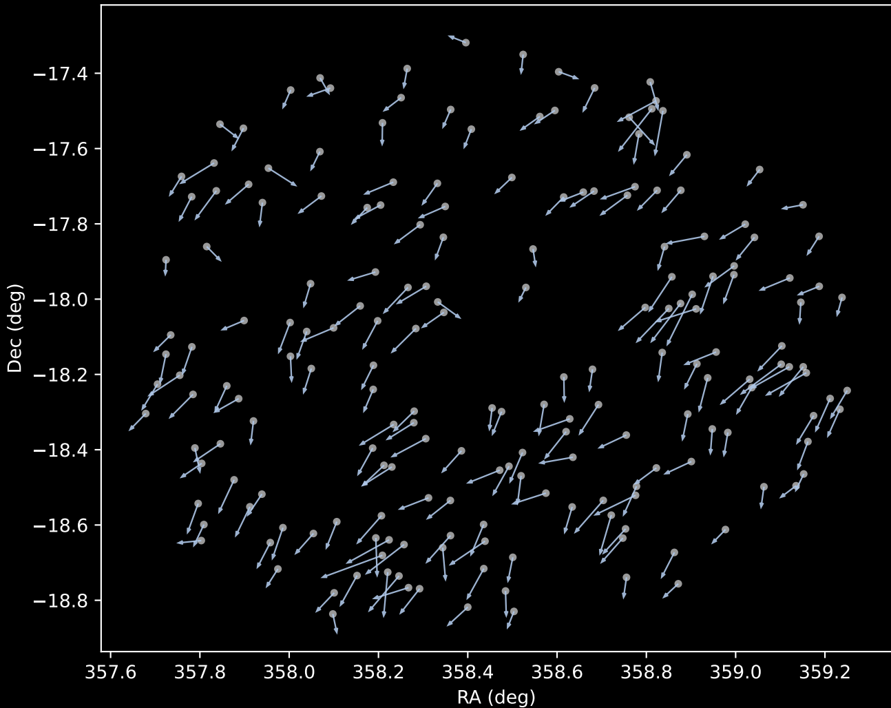
APOGEE DR17 Cluster 1 Proper Motion Vectors (n=193)
