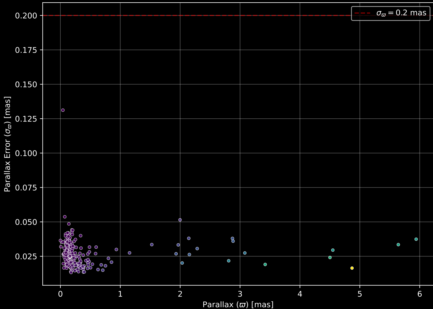
APOGEE DR17 Field: [005+12] Parallax Quality (n= 247)
