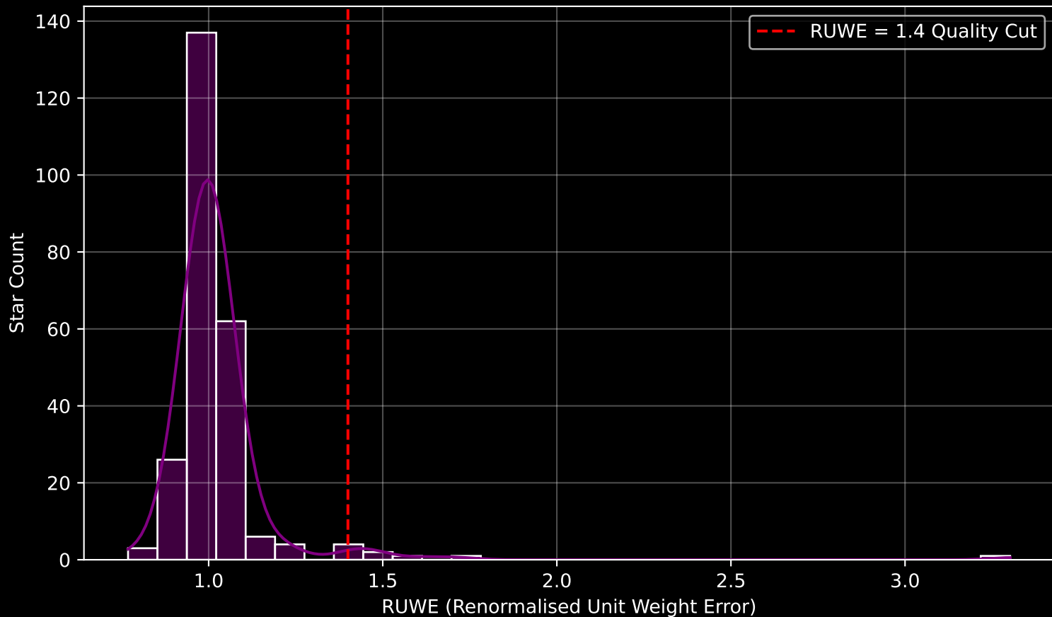
GAPOGEE DR17 Field [005+12] RUWE Distribution (n= 247)
