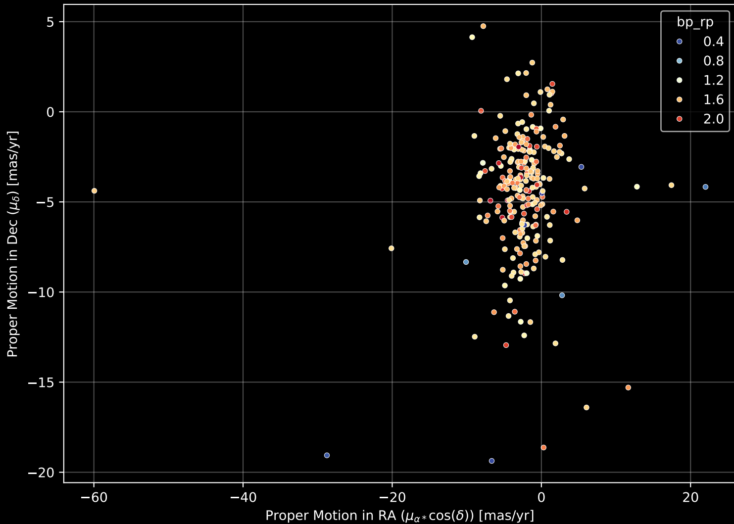
APOGEE DR17 Field: [005+12] Proper Motion Diagram (n= 247)
