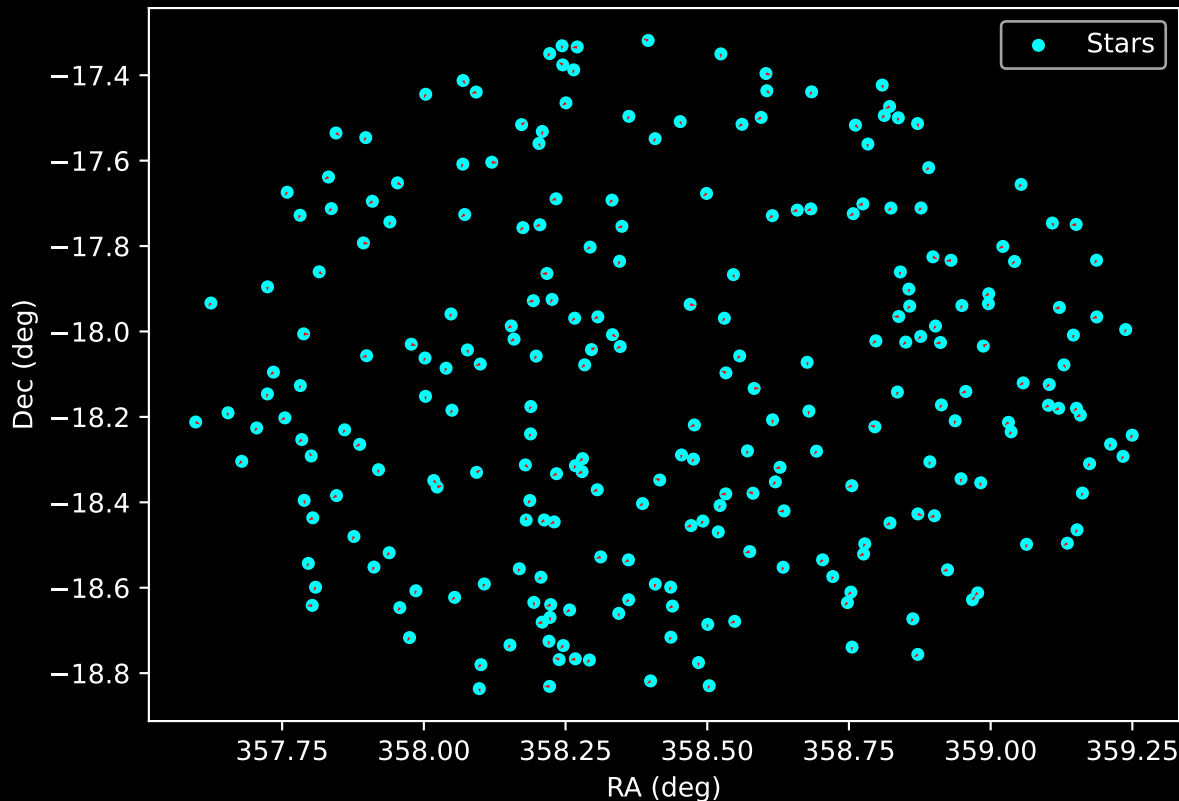
APOGEE DR17 Field: [005+12] Proper Motion Vectors for Gaia Star Field (n= 247)
