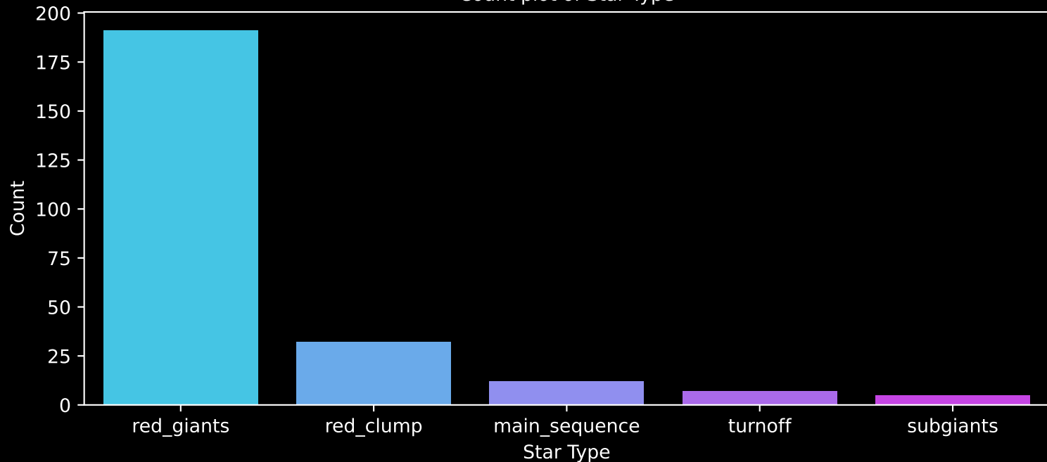
APOGEE DR17 Field: [005+12] Count plot of Star Type
